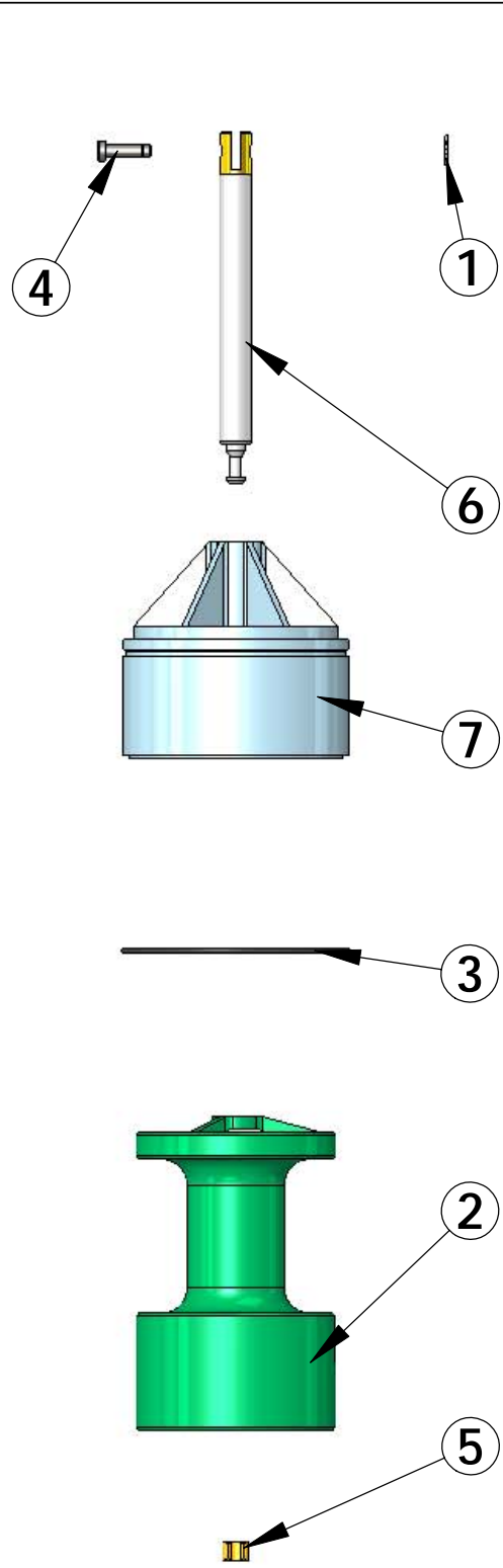
60107-00 W.B.P. PISTON ASSY 3900 LOWER
